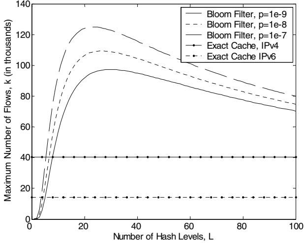
Figure 2: The maximum number of flows that can be stored by a 512KB cache
