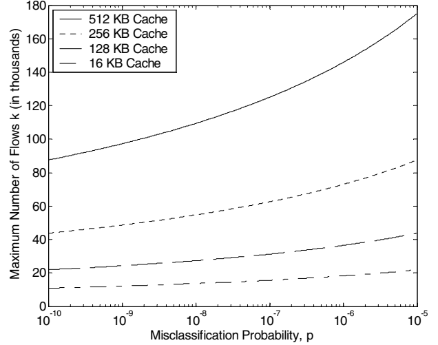
Figure 3: The trade-off between the misclassification probability, p , and the maximum number of elements (flows), k , using optimum values of L .
